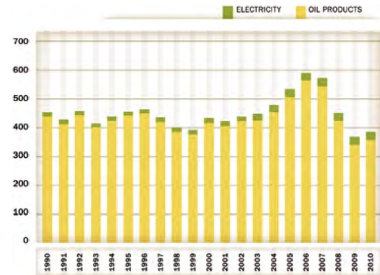
Fig. 46: Railway energy consumption by fuel, 1990-2010 (PJ)
