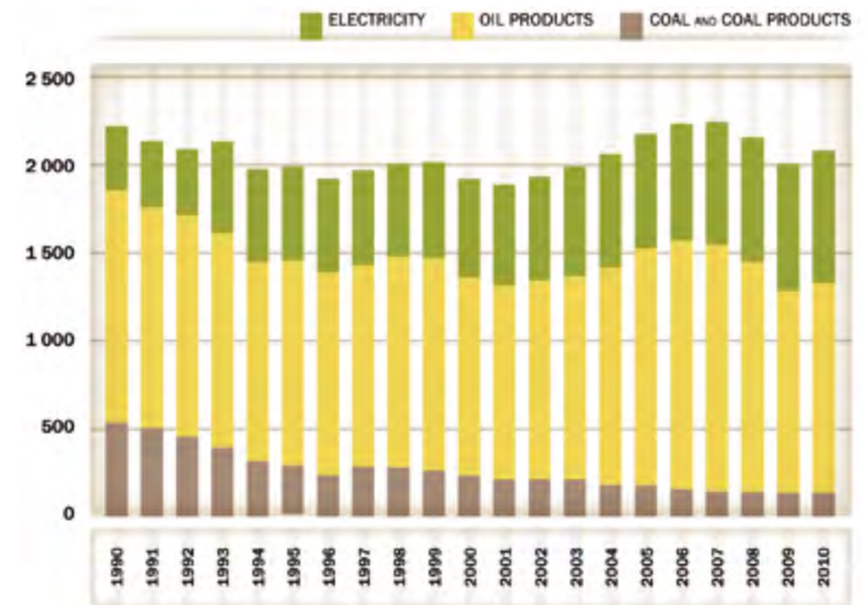
Fig. 16: Railway energy consumption by fuel, 1990-2010 (PJ)
