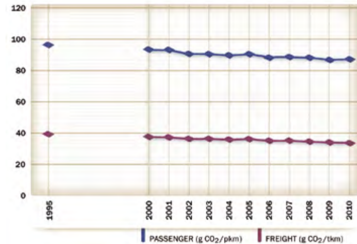
Fig. 73: Railway specific CO 2 emissions, 1995-2010
