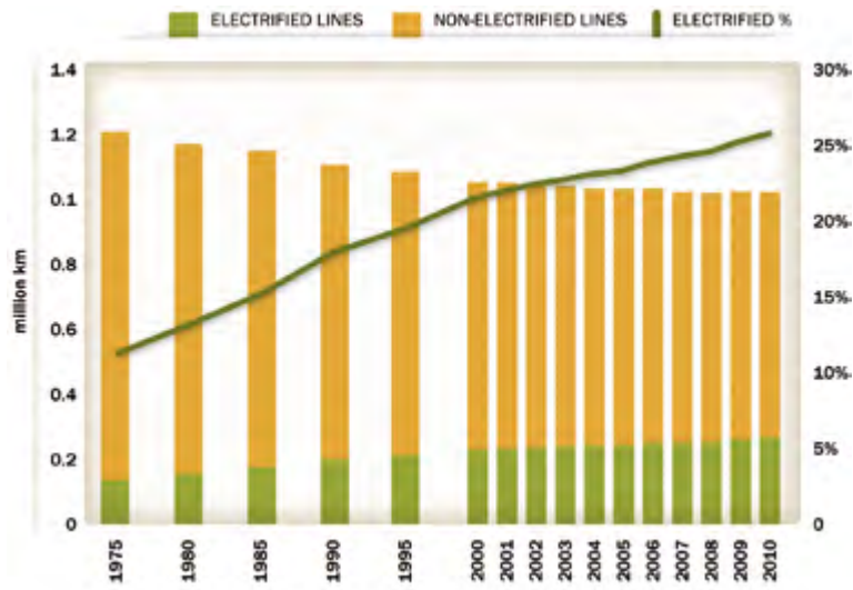
Fig. 10: Length and share of electrified versus non-electrified railway lines, 1975-2010
