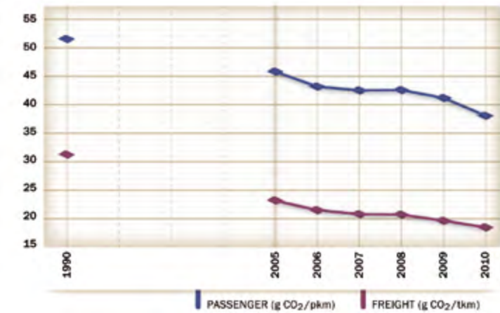
Fig. 39: Railway specific CO 2 emissions, 1990-2010
