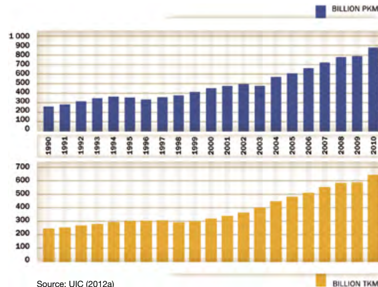
Fig. 87: Passenger and freight railway activity, 1990-2010
