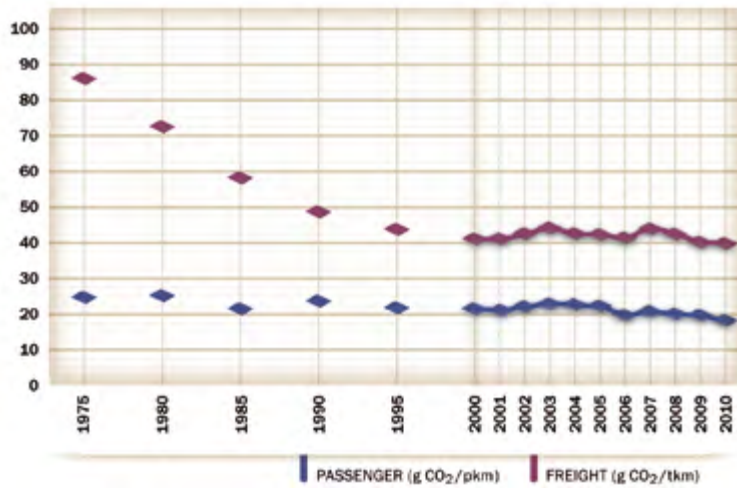
Fig. 63: Railway specific CO 2 emissions, 1995-2010
