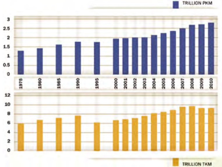
Fig. 2: Passenger and freight railway activity, 1975-2010
