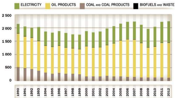
Fig. 16: Railway final energy consumption by fuel, 1990-2012 (PJ)
