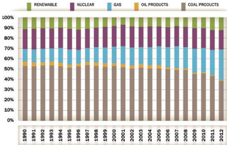
Fig. 43: National electricity production mix evolution, 1990-2012
