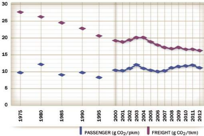
Fig. 93: Railway specific CO 2 emissions, 1975-2012
