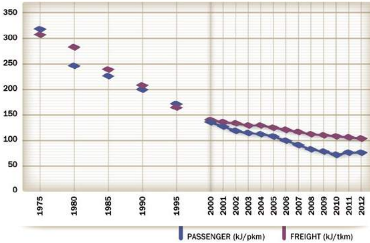
Fig. 80: Railway specific energy consumption, 1975-2012
