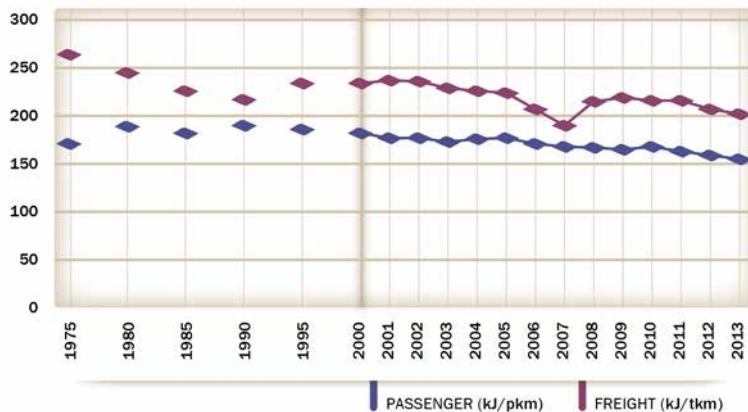
Fig. 52: Railway specific energy consumption, 1975-2013
