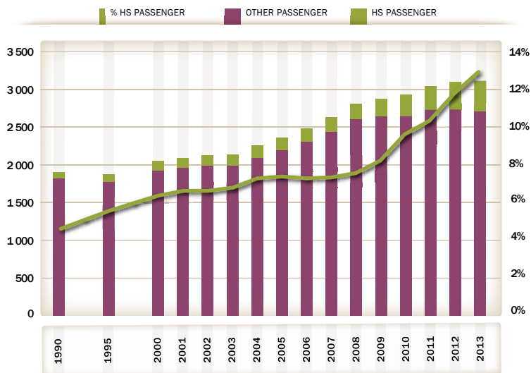
Fig. 12: High-speed activity as a share of total passenger railway activity, 1990-2013 (billion pkm)
