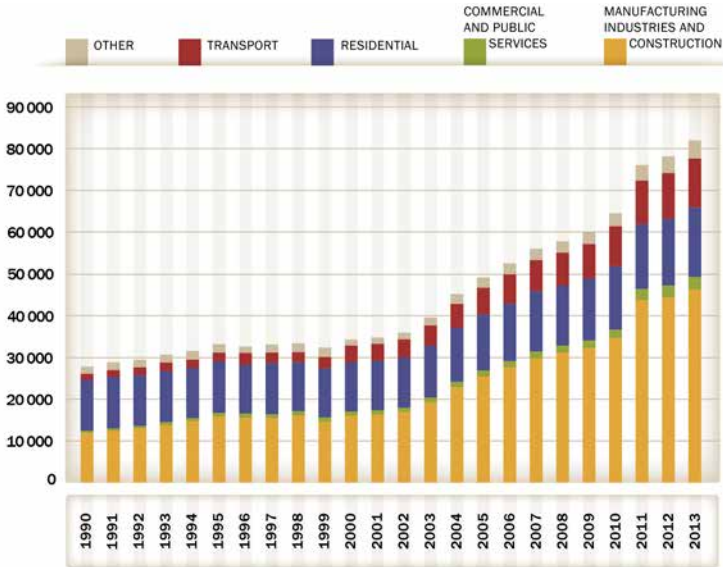
Fig. 81: Total final energy consumption by sector, 1990-2013 (PJ)
