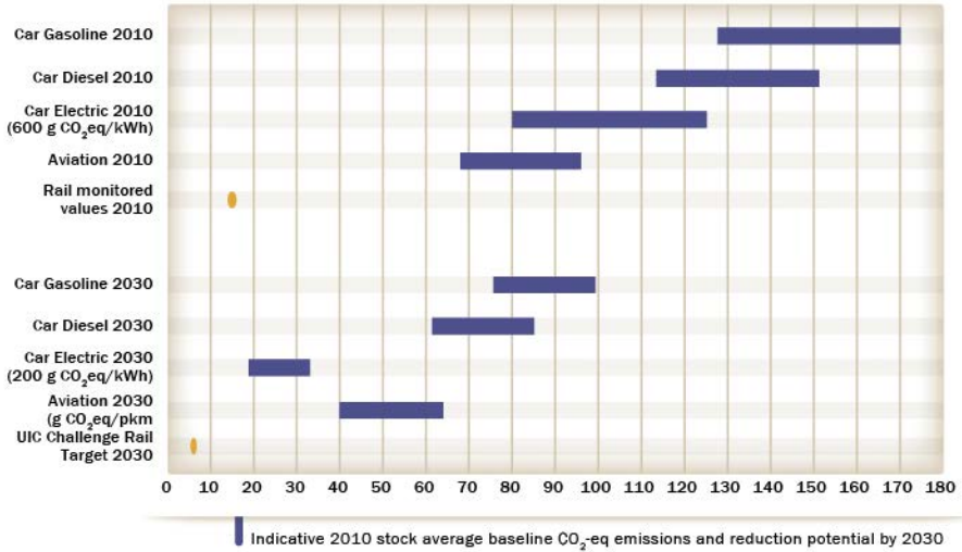
Fig. 96: Comparison between UIC Low Carbon Rail Transport Challenge Targets and CO 2 -eq mitigation potential by 2030 – Passenger (gCO 2 -eq/pkm)
