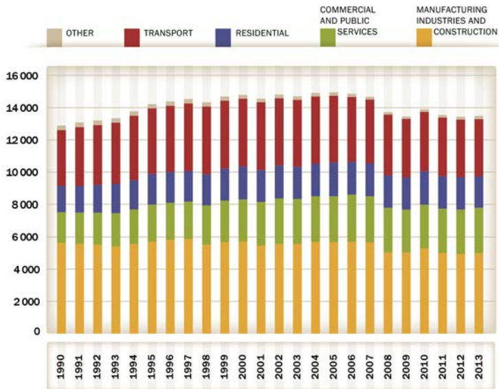
Fig. 45: Total final energy consumption by sector, 1990-2013 (PJ)
