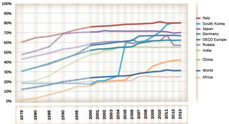
Fig. 9: Share of electrified railway tracks in selected countries and geographic areas, 1975-2013
