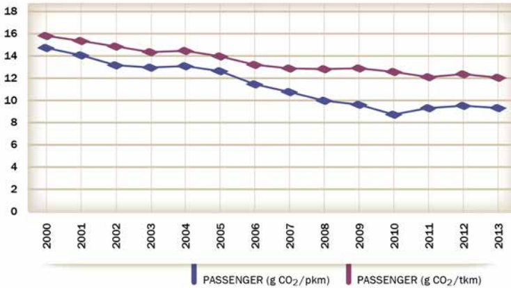
Fig. 77: Railway specific CO 2 emissions, 2000-2013
