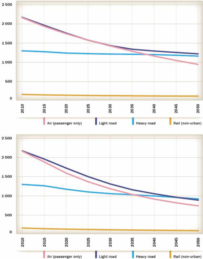
Fig. 101: Specific energy intensity for different modes of transport according to the 4 Degree (top) and 2 Degree (bottom) scenario, (kJ/TU)
