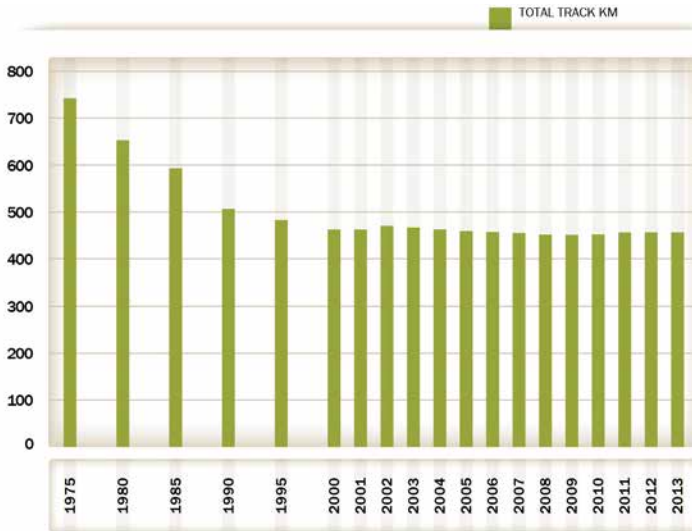
Fig. 37: Length of railway tracks, 1975-2013 (thousand km)
