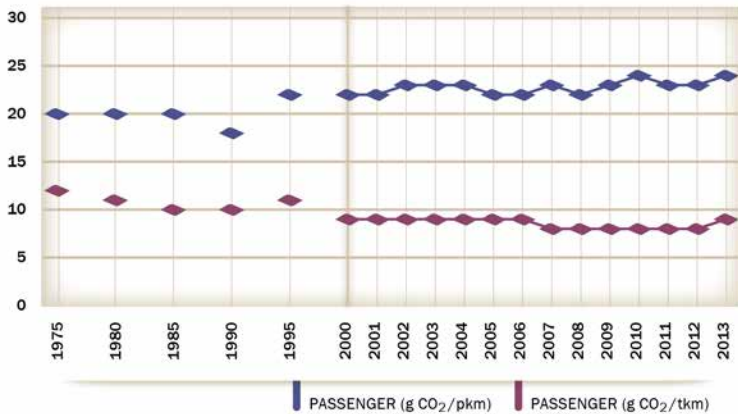
Fig. 65: Railway specific CO 2 emissions, 1975-2013
