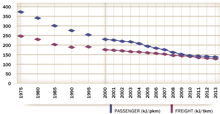
Fig. 15: Railway specific energy consumption, 1975-2013
