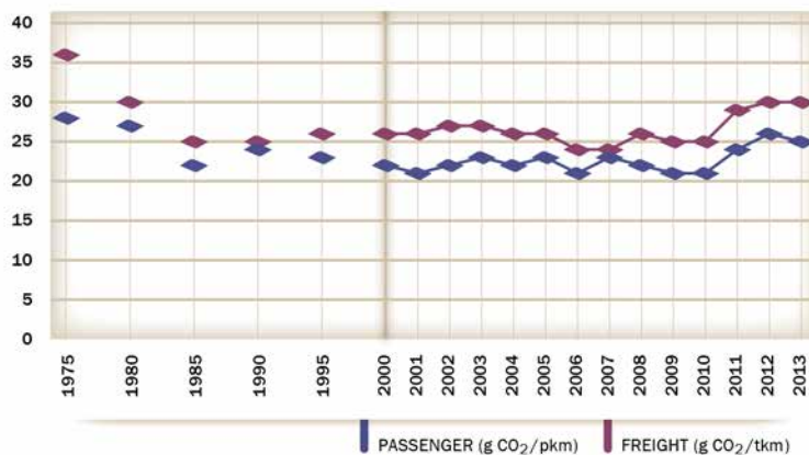
Fig. 53: Railway specific CO 2 emissions, 1975-2013
