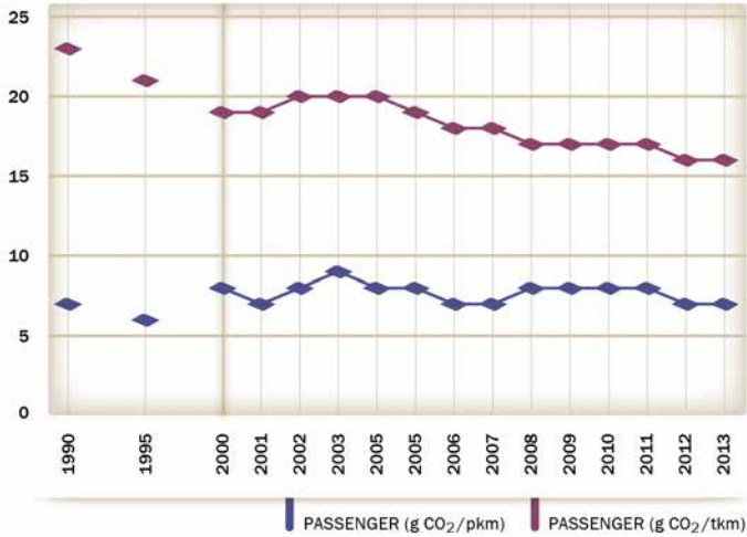
Fig. 89: Railway specific CO 2 emissions, 1990-2013
