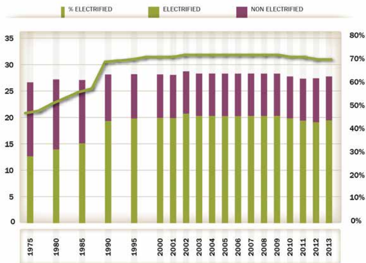
Fig. 49: Length and share of electrified and non-electrified railway tracks, 1975-2013 (thousand km)
