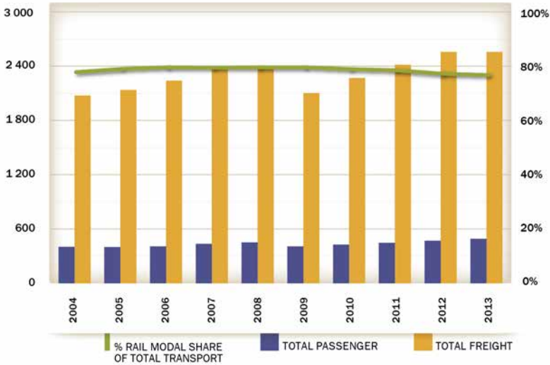
Fig. 59: Passenger and freight transport activity - all modes, 2004-2013 (billion pkm and tkm – left, share of rail over total – right)
