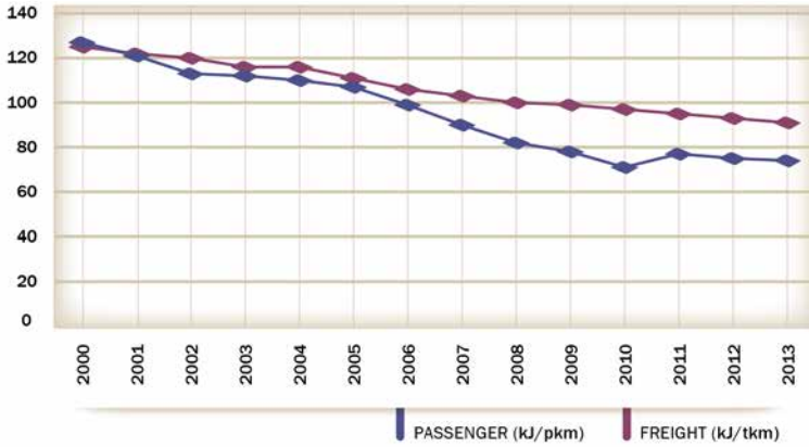
Fig. 76: Railway specific energy consumption, 2000-2013
