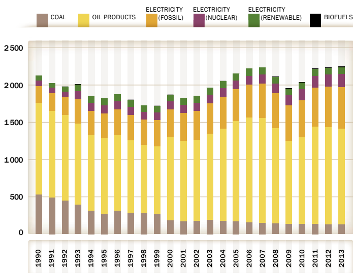
Fig. 13: Railway final energy consumption by fuel, 1990-2013 (PJ)
