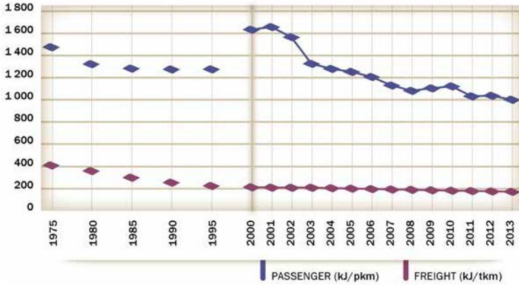
Fig. 40: Railway specific energy consumption, 1975-2013
