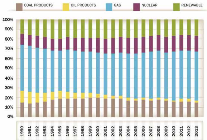
Fig. 63: National electricity production mix evolution, 1990-2013
