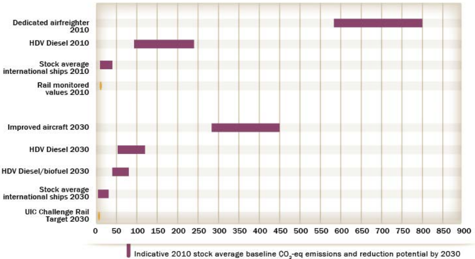
Fig. 97: Comparison between UIC Low Carbon Rail Transport Challenge Targets and CO 2 -eq mitigation potential by 2030 – Freight (gCO 2 -eq/tkm)
