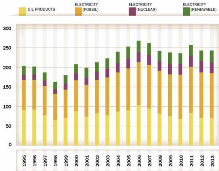
Fig. 62: Railway final energy consumption by fuel, 1995-2013 (PJ)
