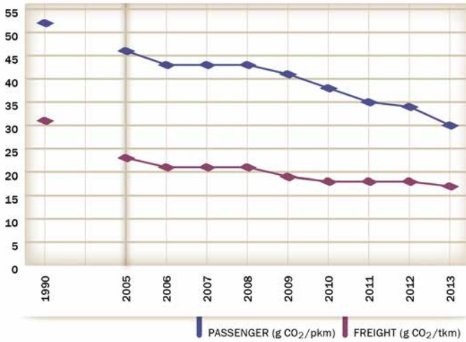
Fig. 29: Railway specific CO 2 emissions, 1990-2013
