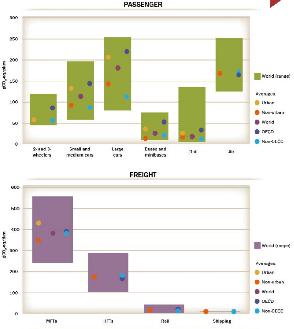
Fig. 98: Current Well-to-Wheel GHG intensities of passenger and freight transport activity, 2015
