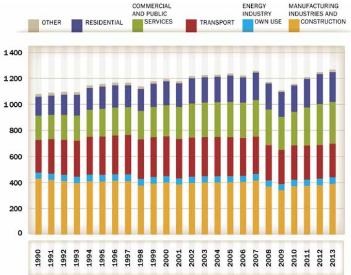
Fig. 43: Total CO 2 emissions from fuel combustion by sector, 1990-2013 (million tCO 2 )
