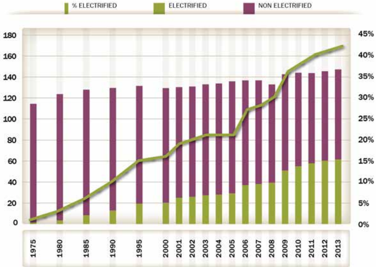
Fig. 85: Length and share of electrified and non-electrified railway tracks, 1975-2013 (thousand km)
