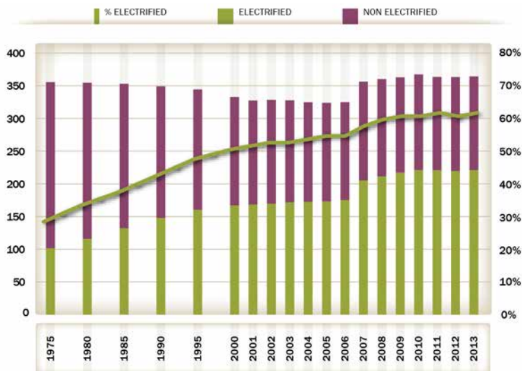
Fig. 24: Length and share of electrified and non-electrified railway tracks, 1975-2013 (thousand km)
