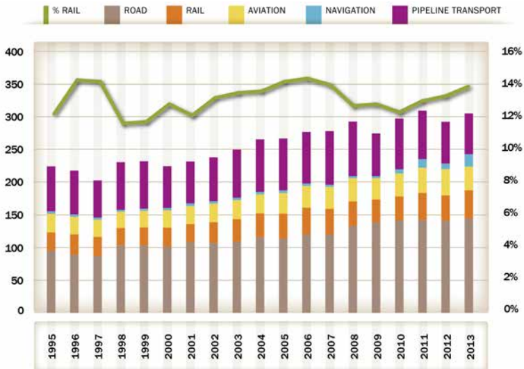
Fig. 58: Transport sector CO 2 emissions by mode, 1995-2013 (million tCO 2 - left, share of rail over total - right)
