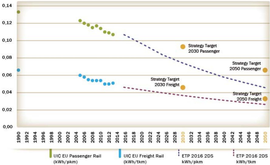
Fig. 92: UIC-Europe Railways specific energy consumption evolution (passenger and freight services) between 1990 and, 2013, compared to UIC-CER 2030 and 2050 targets at EU level
