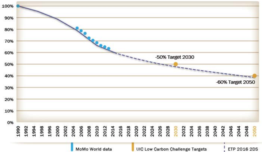
Fig. 90: World specific rail energy consumption evolution per traffic unit (TU) between 1990-2013 compared to 2030 and 2050 targets (1990=100)
