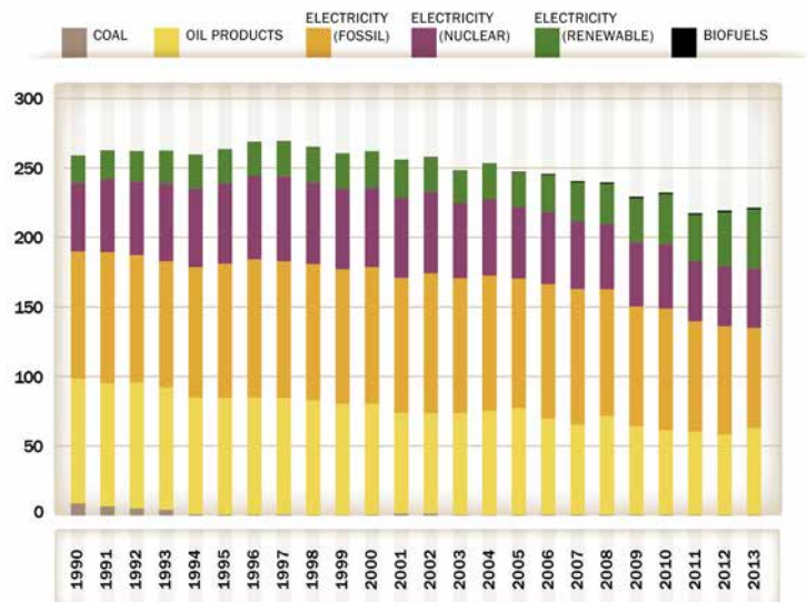
Fig. 25: Railway final energy consumption by fuel, 1990-2013 (PJ)
