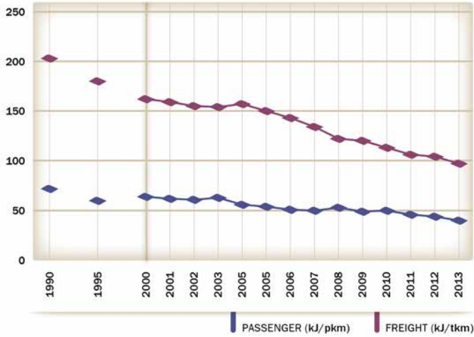
Fig. 88: Railway specific energy consumption, 1990-2013
