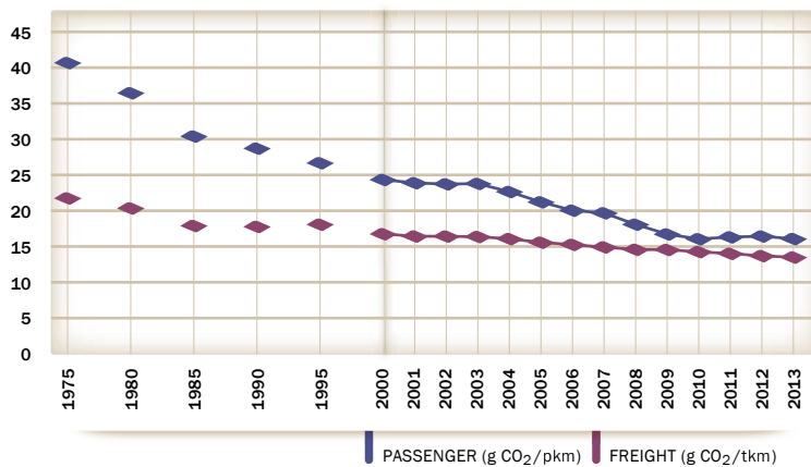
Fig. 16: Railway specific CO 2 emissions, 1975-2013
