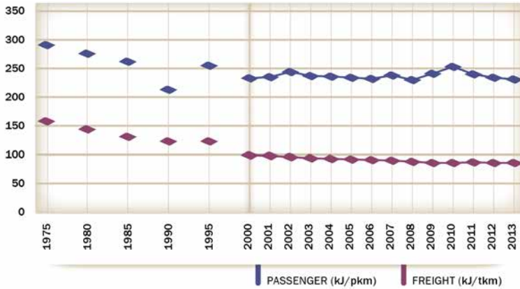
Fig. 64: Railway specific energy consumption, 1975-2013
