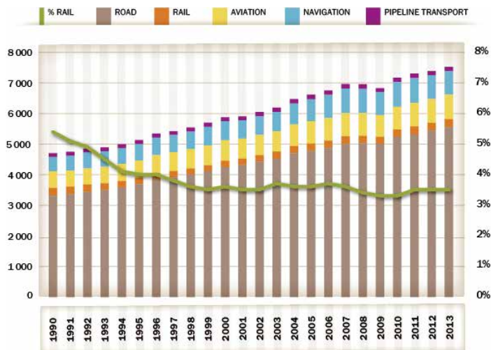
Fig. 5: Transport sector CO 2 emissions by mode, 1990-2013 (million tCO 2 - left, share of rail in global CO 2 emissions - right)
