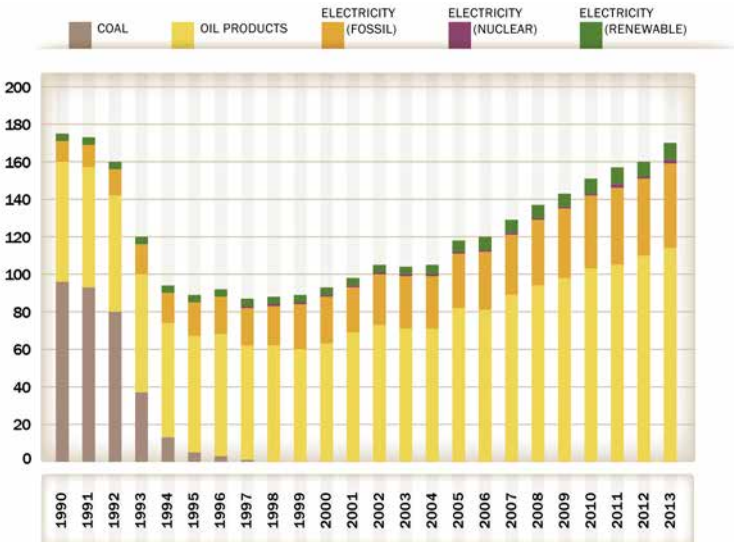
Fig. 74: Railway final energy consumption by fuel, 1990-2013 (PJ)
