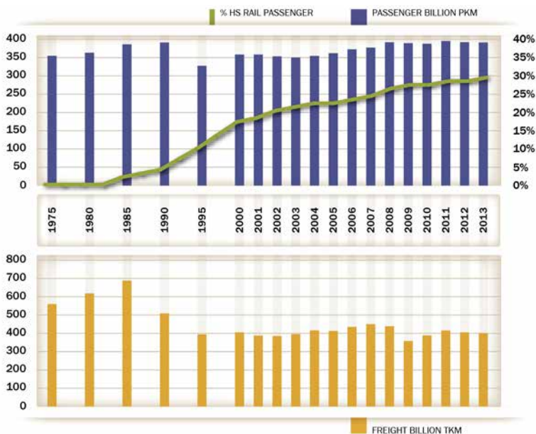
Fig. 23: Passenger and freight railway activity and High-Speed activity as a share of total passenger railway activity (%), 1975-2013
